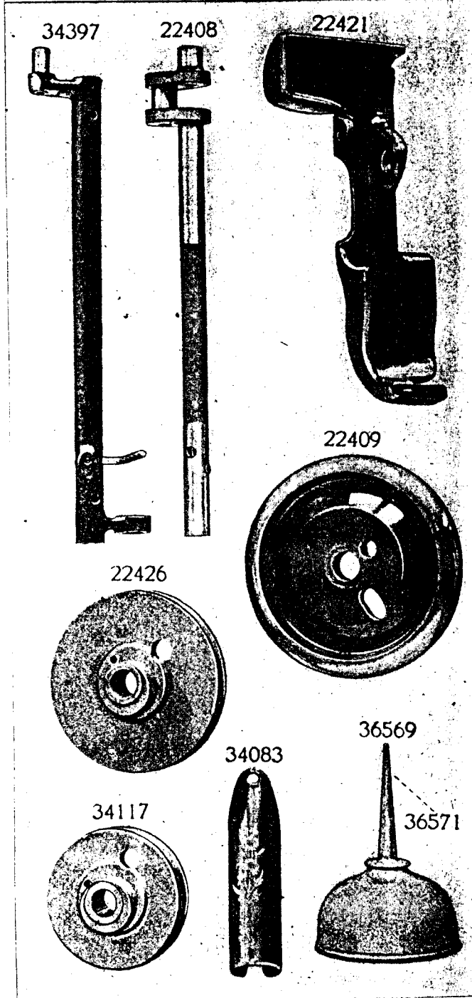
PLATE 6818—ONE-HALF SIZE
