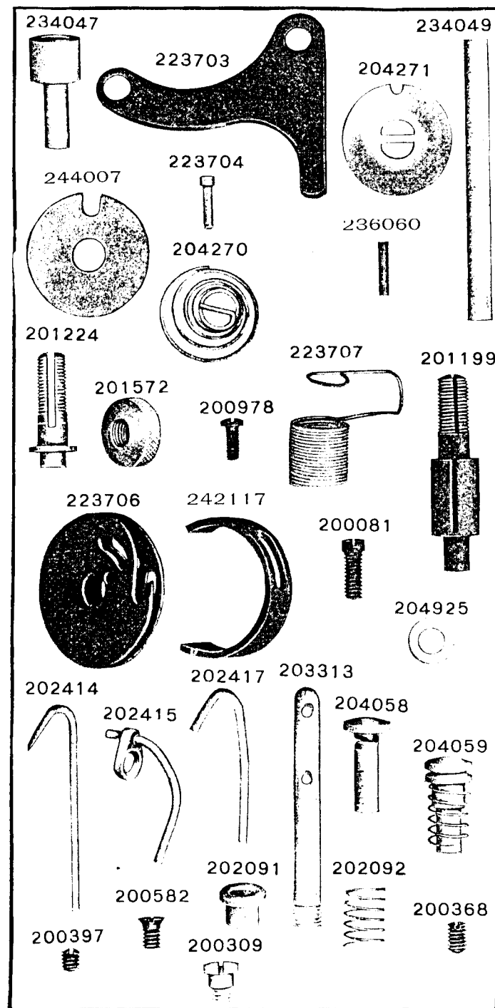
PLATE 13309-FULL SIZE
