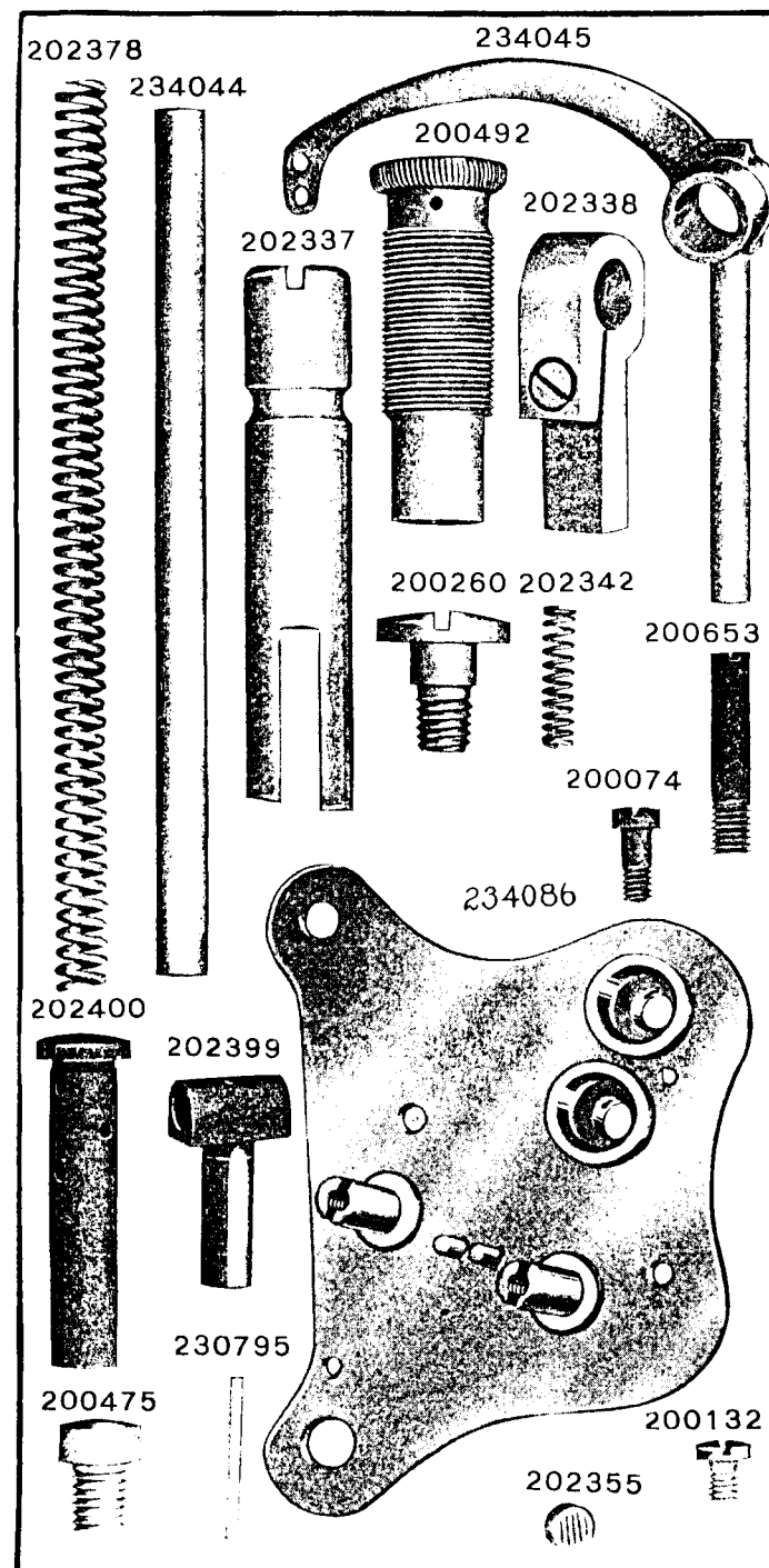
PLATE 13307-FULL SIZE
