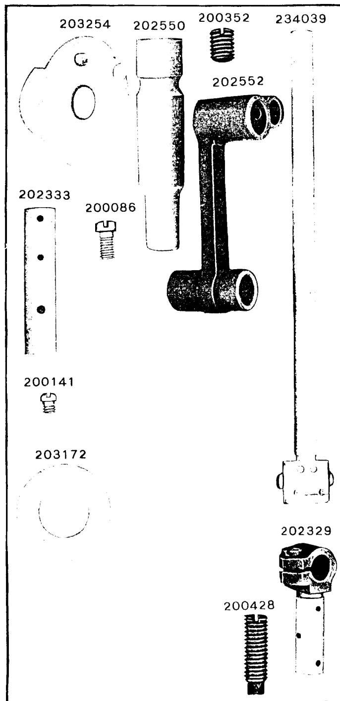
PLATE 13308-FULL SIZE
